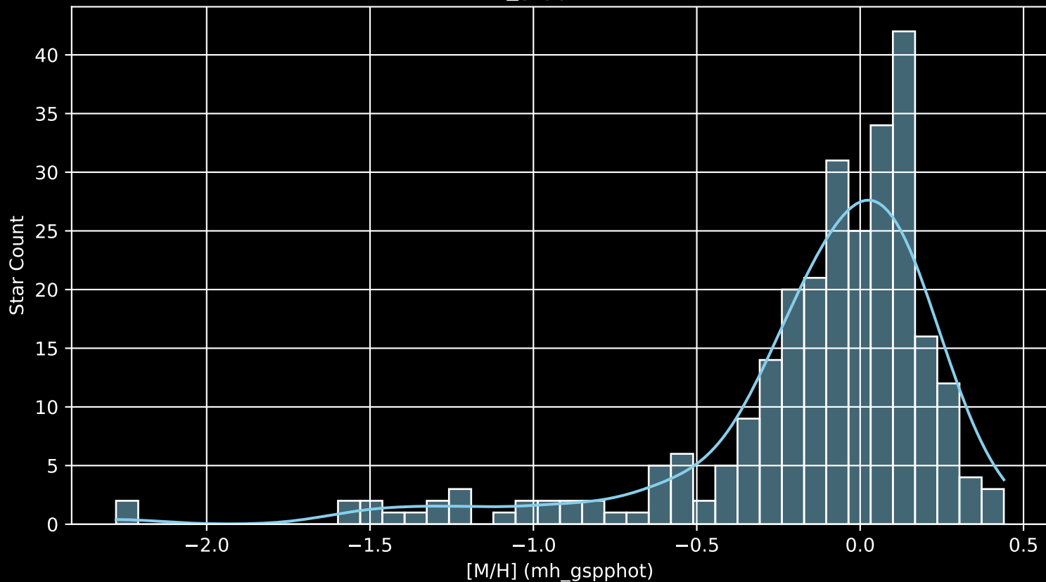
APOGEE DR17 Field: [005-08 [M/H] (mh_gspphot) (n= 273)
