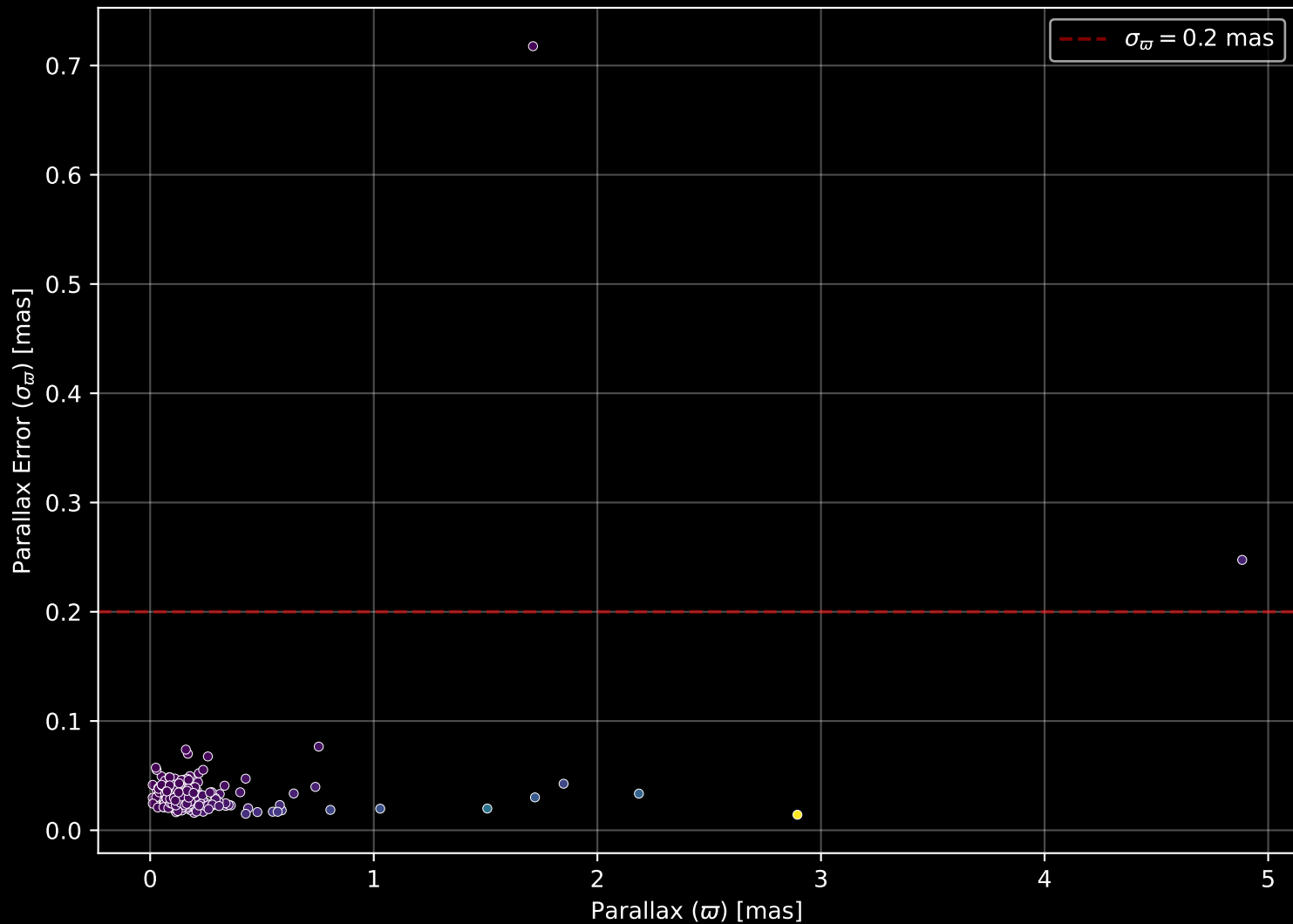
APOGEE DR17 Field: [005-08] Parallax Quality (n= 274)
