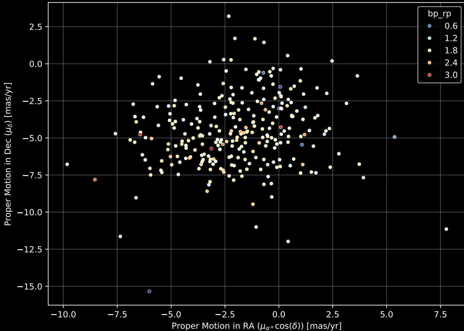
APOGEE DR17 Field: [005-08] Proper Motion Diagram (n= 274)
