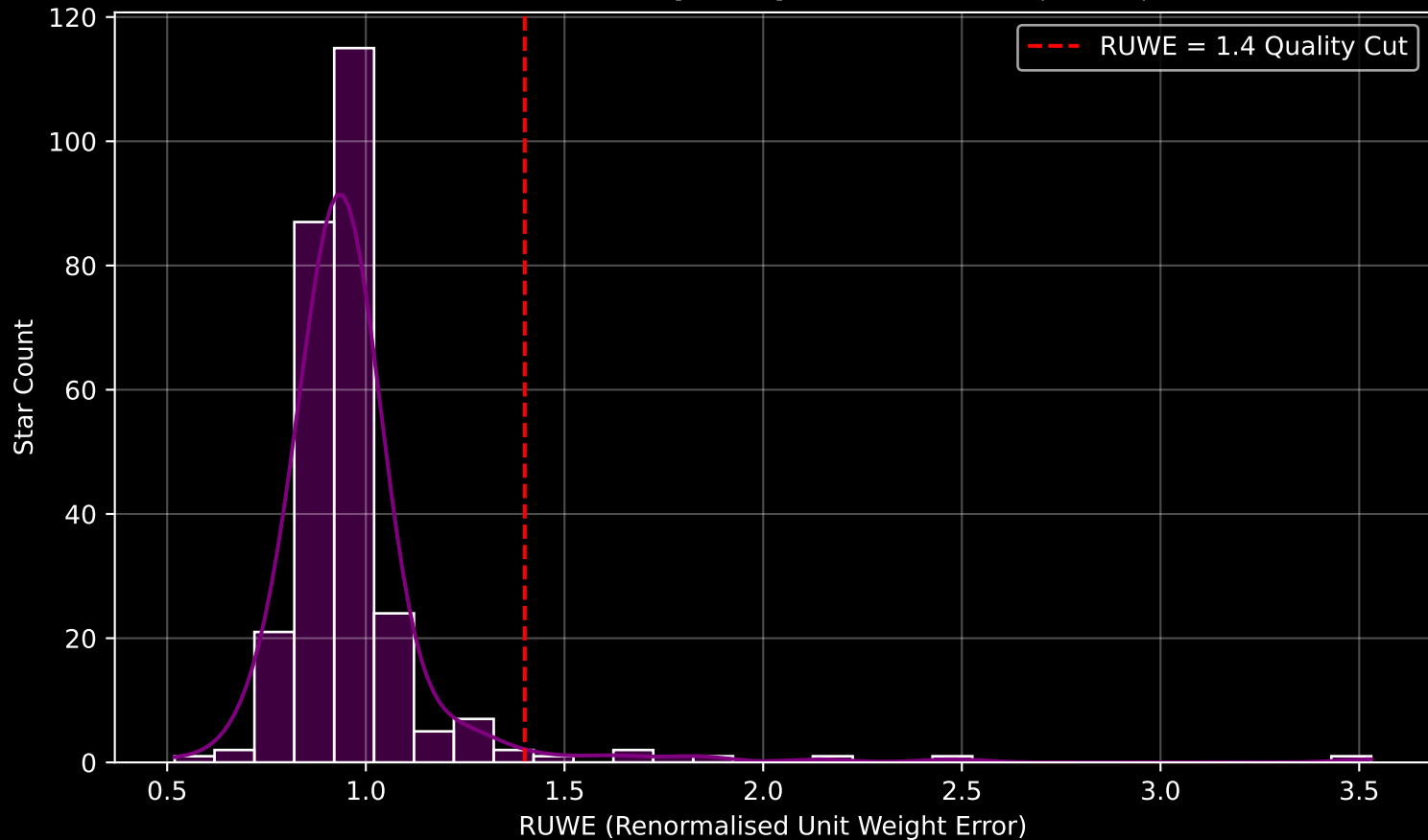
GAPOGEE DR17 Field [005-08] RUWE Distribution (n= 272)
