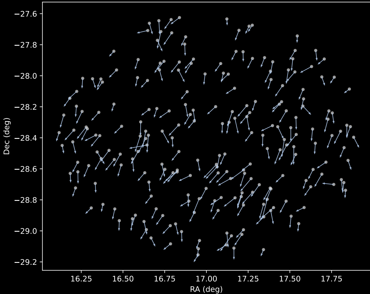
APOGEE DR17 Cluster 1 Proper Motion Vectors (n=223)
